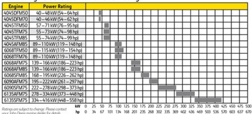
Marine Engine Generator Drive Power Ratings
